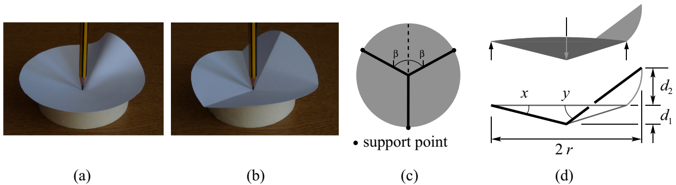
FIG. 3. Deformation of a d-cone. (a) Continuous d-cone. (b) Discrete d-cone. (c) Fold line layout for panel (b) where \beta is the half-width of the elevated portion above the rim. (d) Schematic side-view of the deformed discrete d-cone showing the upward support forces and centrally applied downward force. The bottom subfigure shows true views of the valley and mountain folds along the diameter in panel (c), which are rotated by angles x and y from the horizontal plane. The “conical indentation” from Ref. [5] is the displacement of the center, d_1 , and the upwards buckled displacement is d_2 .
