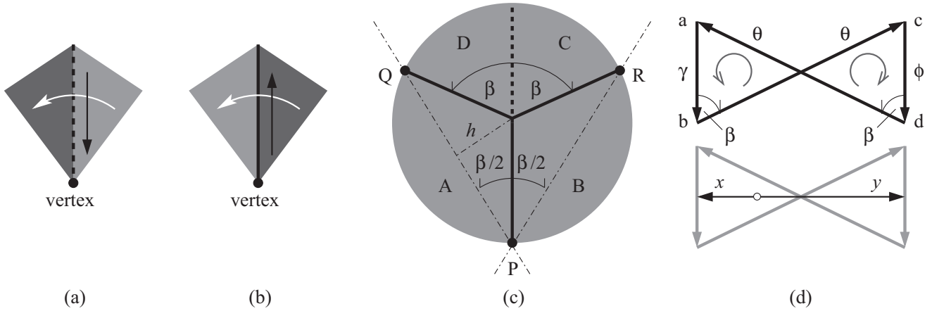
FIG. 4. Kinematics of a discrete d-cone. The direction of positive fold rotations as vectors along a mountain fold, panel (a), and valley fold, panel (b), when moving counterclockwise around the vertex. (c) Like Fig. 3(c) but indicating the four facets A, B, C, and D between fold lines, the three support points P, Q, and R, and the support lines, PQ and PR. h is the perpendicular lever arm about PQ for calculating the displacement of the center. (d) The Gauss mapping for the rotation vectors along the fold lines: ab = \gamma pertains to a rotation, \gamma , between facets A and B, and so forth for \theta (bc and da) and \phi (cd). The internal curved arrows show the vector circuit when assessing the sign of the enclosed area. The bottom subfigure shows how to relate x and y from Fig. 3(d).
