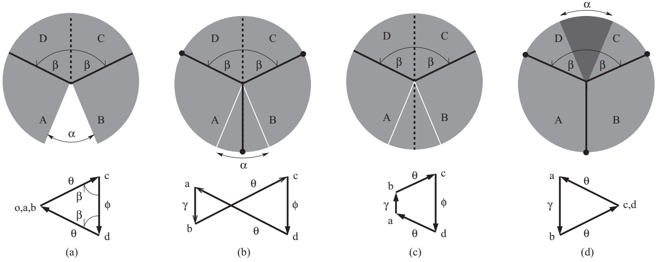
FIG. 5. Gauss's mapping for the various folded shapes from Fig. 2. (a) The planar confined e-cone. (b) The conically confined e-cone. (c) The free-standing e-cone. (d) The p-cone. In all, the angular excess or deficit of the central vertex is of magnitude \alpha . The fold notation and nomenclature are the same as described in the captions of Figs. 2 and 4.
