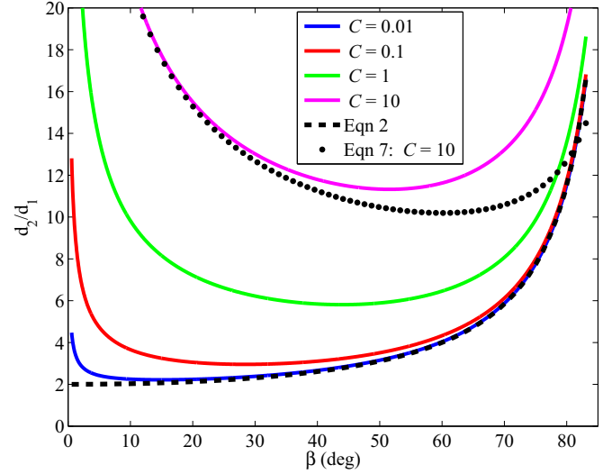
FIG. 6. Discrete e-cone displacements. C is equal to \alpha/\gamma^2 and measures the influences of angular excess and conical indentation: a large value ( \gg 1 ) of C is close to the planar e-cone case, Eq. (7), while a small value ( \ll 1 ) approaches d-cone behavior, Eq. (2). \beta can extend up to 90^\circ , but all curves rise asymptotically and diminish the earlier detail, hence the abscissa range as shown. The solid curves are exact solutions using Eq. (6).
